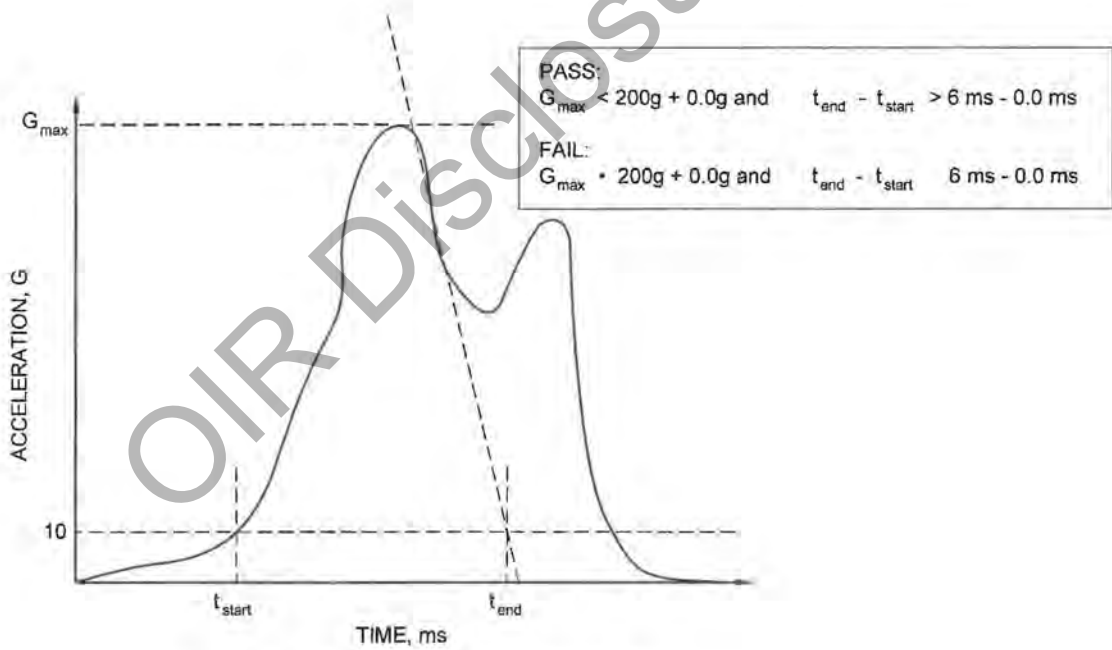
(b) Example of a multi-peak acceleration impulse
