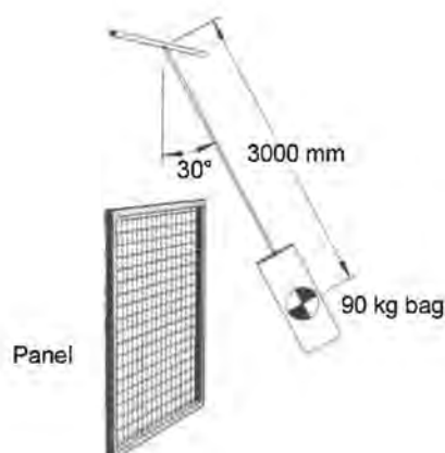
FIGURE E1 BARRER TEST METHOD
